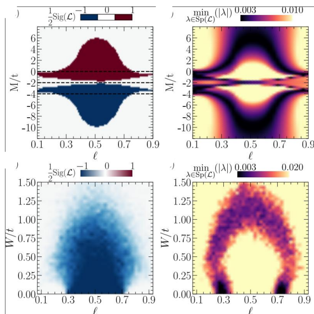
Figure 1: Topological phase diagrams for undistorted and distorted members of the Hat family. Given by the spectral localizer and its local gap.
