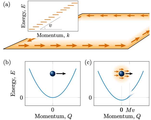
Figure 1: Chiral dressing of a mobile impurity injected on the edge of a topological insulator. (a) The edge of the topological insulator provides a chiral mode, with linear dispersion relation E = vk (b) We inject a mobile impurity of mass M and momentum Q on the edge of the system. In the absence of interactions with the chiral bath, its dispersion relation is quadratic (free particle). (c) Upon activating interactions, the impurity is dressed by the chiral bath. Its spectral function displays a chiral behavior with strong bath-impurity coupling features at momenta of the order of Mv , a clear signature of the chiral dressing.
