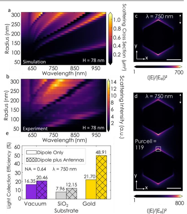
Figure 1: WS 2 hexagonal nanoantennas on gold optical characterisation and simulation. (a) and (b) show simulated and experimental scattering spectra of monomers of height 78 nm for a range of radii respectively. (c) and (d) show the top view of the electric field intensities for a monomer and dimer respectively, each with height 180 nm and radius 120 nm. White double-headed arrow shows excitation polarisation. Purcell factor is from a dipole placed 0.5 nm above the inner dimer vertex, highlighted by the white box, where the electric field is maximised. Scale bars are 100 nm. (e) shows the light collection efficiency in simulation of a dipole placed 0.5 nm above different substrates, compared to a dipole 0.5 nm above the inner dimer vertex. The numerical aperture used is 0.64 with dipole polarisation along the dimer axis and wavelength 750 nm.
