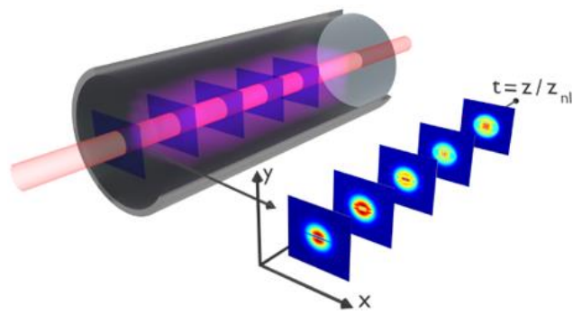
Figure 1: Scheme of laser beam propagating through atomic vapor (nonlinear medium) resulting in the simulation of a 2D fluid of light while propagation axis ( z ) corresponds to the time evolution of this fluid.
