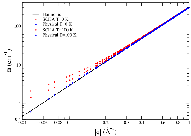
Figure 1: Frequency of the ZA mode in the harmonic approximation, within the SCHA and obtained from the Hessian of the SCHA (labeled as "Physical") both at 0 K and 100K using the membrane model. The physical phonons recover the quadratic dispersion of the harmonic solution.
