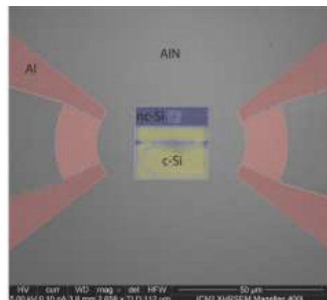
Figure 1: The core of the PHENOMEN platform. Left and right in orange depict the interdigitated electrodes for launching and detecting surface acoustic waves. The central square is the heart of the circuit. It includes a nanobeam actuated by a waveguide running in parallel and with a photonic crystal mirror termination. This platform was demonstrated at 1 GHz [6] and 2 GHz (To be published).
