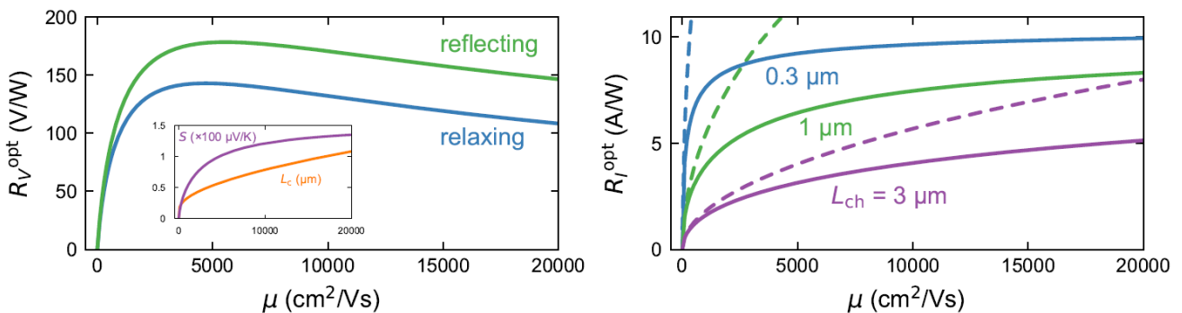
Figure 1: Optimal photovoltage (left) and photocurrent (right) as a function of graphene carrier mobility. In both cases, the photoresponse saturates for a mobility around 5000 \text{ cm}^2/\text{Vs} .
