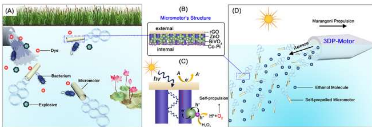
Figure 1: Schematic illustration of (A) versatile micromotors dynamically degrading dyes and explosives and killing bacteria in contaminated water, (B) structure of the designed micromotor, (C) design strategy of Co-Pi/ \text{BiVO}_4 / \text{ZnO} /rGO: (i) increased light absorption and charge generation in both \text{BiVO}_4 and \text{ZnO} through light trapping effect of the nanorods, (ii) electron injection into \text{ZnO} nanorods followed by prompt electron transport along \text{ZnO} nanorods, (iii) electron collection and storage in rGO for reduction reaction and (iv) hole transfer to Co-Pi for efficient water oxidation to generate oxygen bubbles for self-propulsion of micromotor, (D) 3D-printed millimeter-scale motor releasing micromotors and ethanol molecules.
