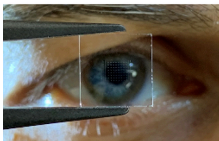
Figure 1: Left: transparent image sensor based on an array of graphene photodetectors. Right: eye-track device
