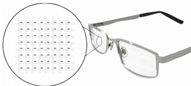
Figure 1: Left: transparent image sensor based on an array of graphene photodetectors. Right: eye-track device
