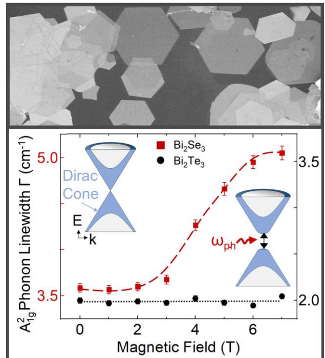
Figure 1: Upper panel: SEM micrograph of \text{Bi}_2\text{Se}_3 nanoflakes. Lower panel: Linewidth dependence of the A_{1g}^2 phonon of both materials as a function of magnetic field showing a larger effect of the field on the \text{Bi}_2\text{Se}_3 phonon. The inset cartoons show the change in the energy dispersion of a TI with applied magnetic field. The linewidth changes in the \text{Bi}_2\text{Se}_3 phonon above 3 T are explained by a coupling to an electronic transition from the lower to the upper gapped Dirac Cone.
