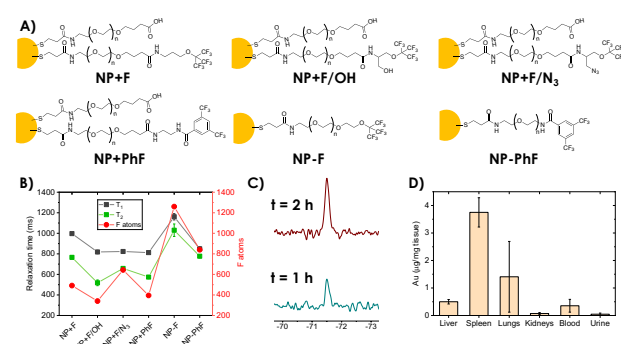
Figure 1: A) Fluorinated NPs prepared. B) Plot of relaxation times and number of fluorine atoms. C) in vivo ^{19}\text{F} MRS at 1 and 2 hours. D) ICP-MS analysis of extracted tissues and organs.
