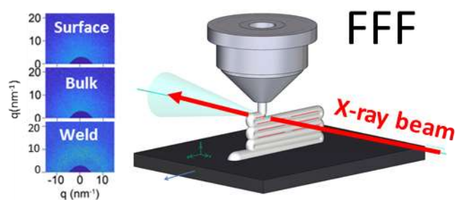
Figure 1: Conceptual view of the experimental approach followed to investigate in real time structure development during Fused Filament Fabrication (FFF)[3].
