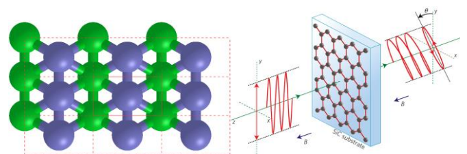
Figure 1: Electronic and optical properties of borophene and strained graphene
