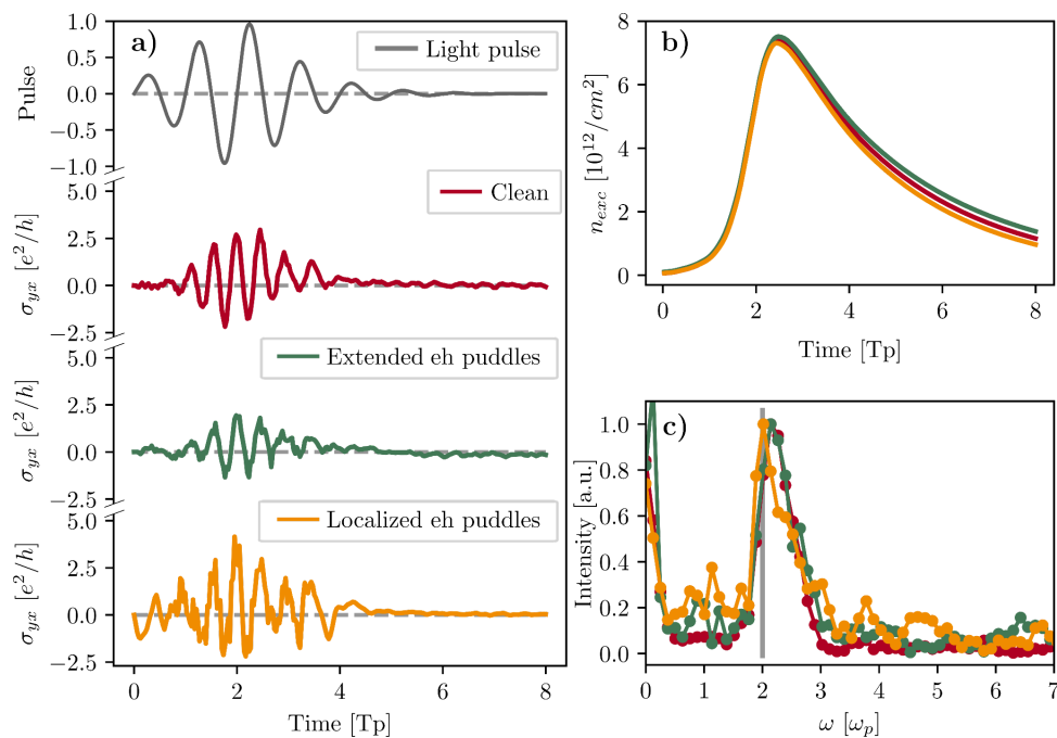
Figure 1: a) Time dependence of the applied light pulse in gray, and the Hall conductivity in red, green, and yellow for the clean system, extended and localized electron-hole puddles, respectively. b) Number of excited carriers c) Fourier transform of the time-dependent conductivity.
