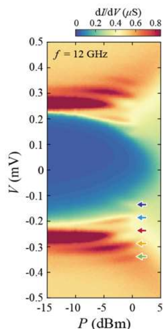
Figure 1: Microwave power dependence of Floquet-Andreev states
