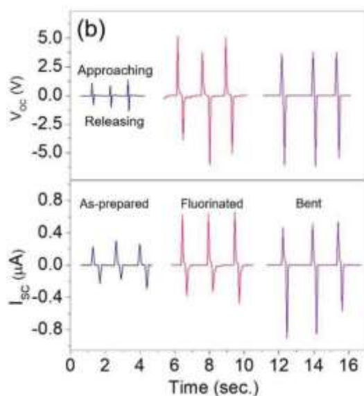
Figure 1: Open-circuit voltage and closed-circuit current of graphene based TENG with fluorinated PDMS, in addition to the effect induced by bending the TENG device [4].
