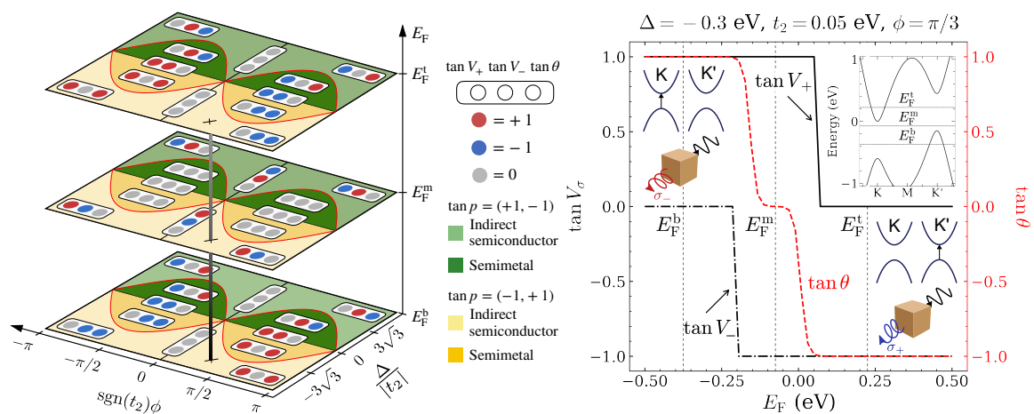
Figure 1: (Left) Optical phase diagram of the modified Haldane model [2]. Circular dichroism, valley polarization and pseudospin polarization is represented by the values \tan \theta , \tan V_\sigma and \tan p , respectively. (Right) Tunability of circular dichroism and valley polarization with varying Fermi energy.
