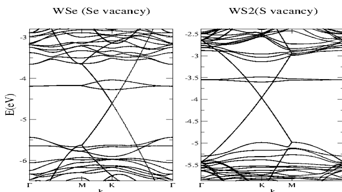
Figure 2: Electronic Band structure for WSe2 and WS2 with a vacancy in the TMDC.
