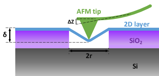
Figure 1: Typical nanoindentation experiment.
