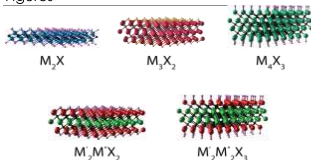
Figure 1: Schematic representation of various MXene structures including M_2X , M_3X_2 , M_4X_3 and the ordered Double-M MXenes ( M'_2M''X_2 and M'_2M''_2X_3 ). M represent a transition metal including, Sc, Ti, Zr, Hf, V, Nb, Ta, Cr, and Mo, and X represent C or N. MXene surfaces are terminated with -O , -OH , -F . M' and M'' in the bottom schematics represent two different transition metals (e.g., Mo and Ti in Mo_2TiC_2 ).
