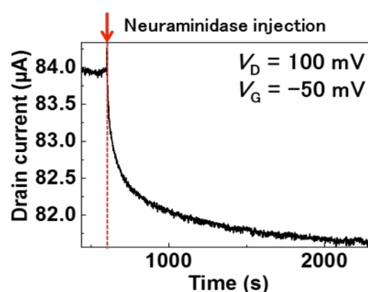
Figure 2: Time dependence of neuraminidase reaction monitored by graphene FET
